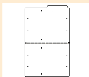
Fastener attachment positions (8 points)
